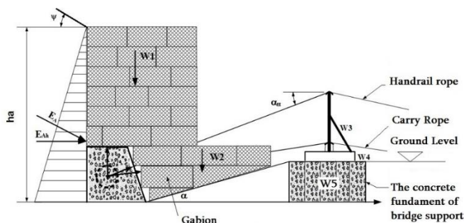
Fig. 3. The device of the "gravitational" anchor of the bearing cable of the suspension bridge using gabions.
