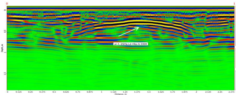
Fig. 2. Radarogram of a sphere with a vertical metal cylinder turned on, the in-phase axes show the presence of a rigidly reflecting object surface at the upper part of the radio image with clear bright lines.
