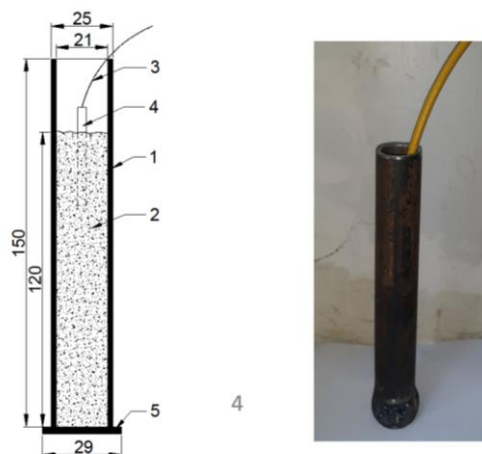
Fig.3 Diagram (a), and view (b) of testing tube of synthesized "molecular compounds"
