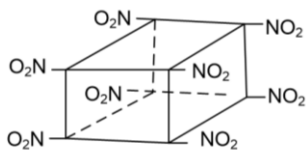
octanitrocubane
