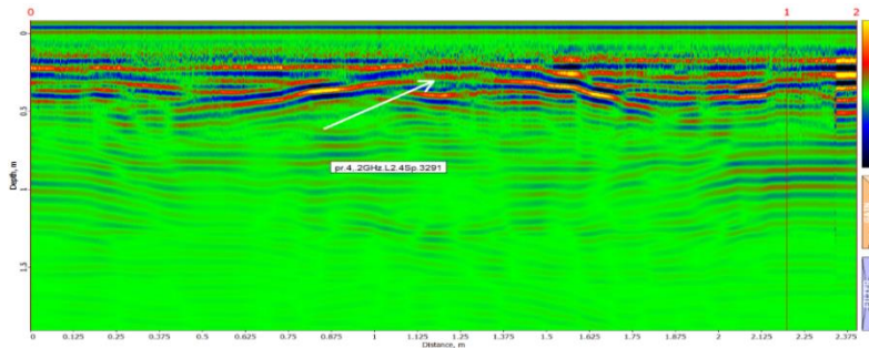
Fig. 1. Radarogram of a hollow sphere, the in-phase axes show the presence of a cavity at the upper part of the radio image with burred lines.
