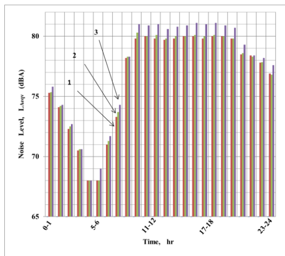
Fig.2 - changes in equivalent to noise level L_{Aeqv} with one-hour time intervals during day and night between the cross-roads of Tornike Eristavi street.
