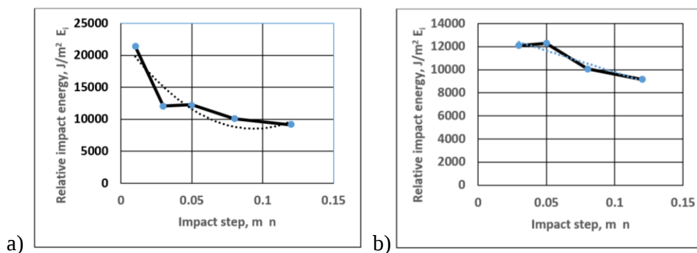
Fig. 1. Relationship graph between relative impact energy and Impact step (a) I-V variant; b) II-V variant).
